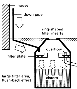
7 In-flow filter
